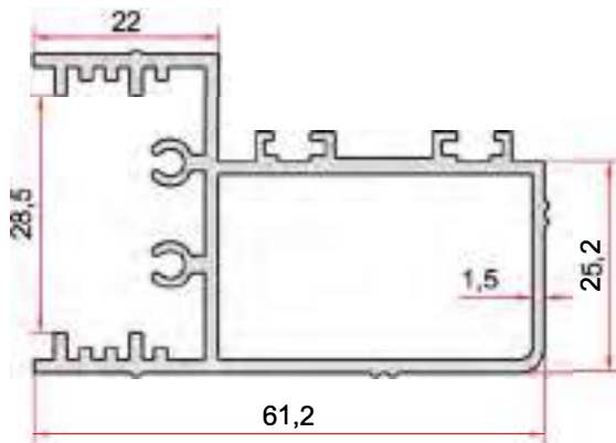
KOD-CODE TEORİK AĞIRLIK EP-2631 THEORETICAL WEIGHT 0,726 Kg/m
