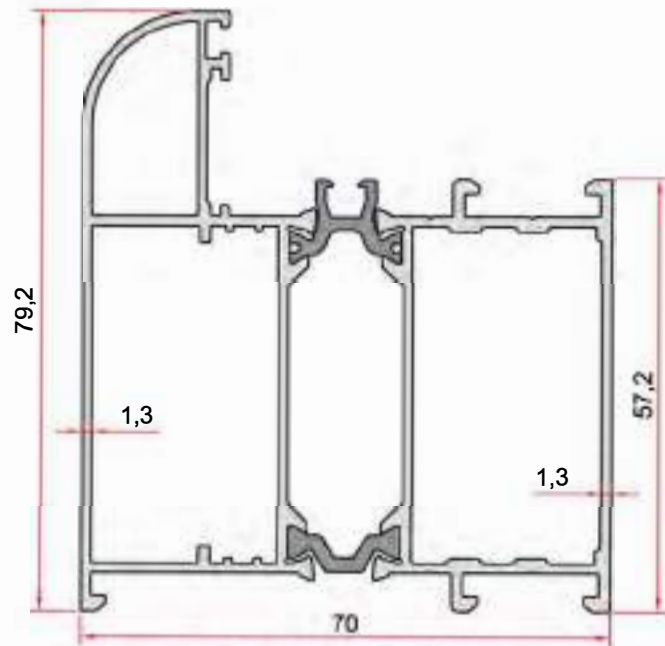
KOD-CODE TEORİK AĞIRLIK THEORETICAL WEIGHT EPAT-7002-13 1,757 Kg/m
