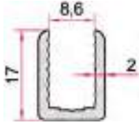
KOD-CODE TEORİK AĞIRLIK THEORETICAL WEIGHT EP-5001 0,213 Kg/m
