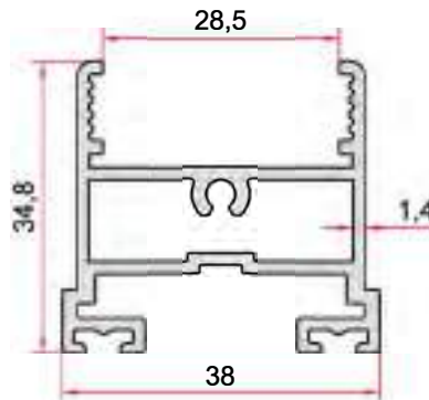
KOD-CODE TEORİK AĞIRLIK EP-2634 THEORETICAL WEIGHT 0,726 Kg/m
