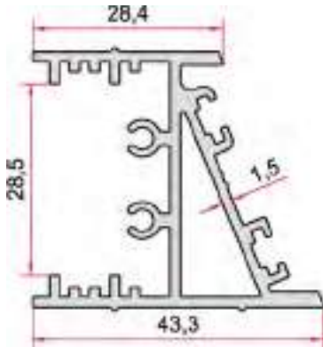
KOD-CODE TEORİK AĞIRLIK EP-2633 THEORETICAL WEIGHT 0,843 Kg/m
