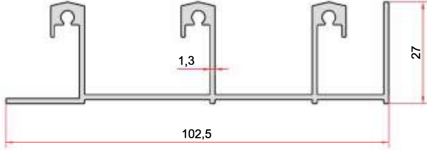
KOD-CODE TEORİK AĞIRLIK EP-7032 THEORETICAL WEIGHT 1,000 Kg/m
