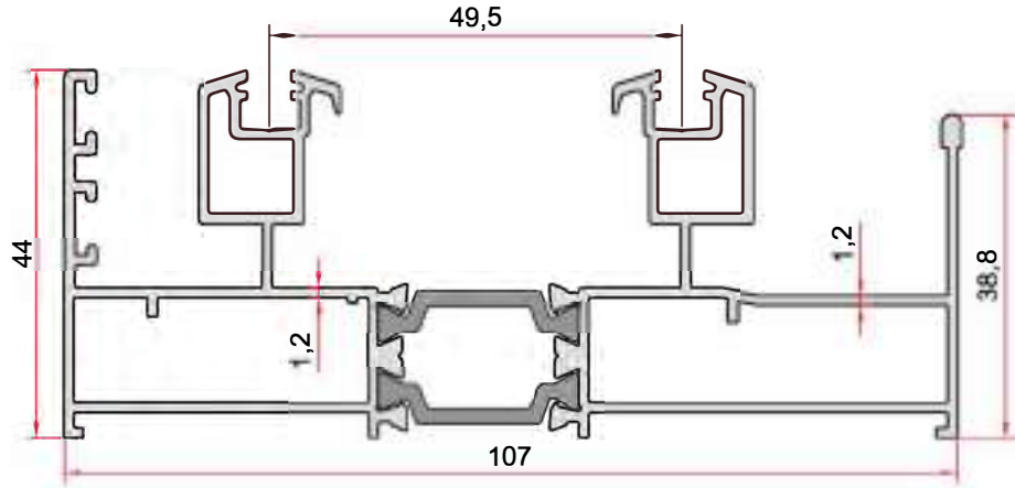
KOD-CODE TEORİK AĞIRLIK EPMD-103-12 THEORETICAL WEIGHT 1,825 Kg/m
