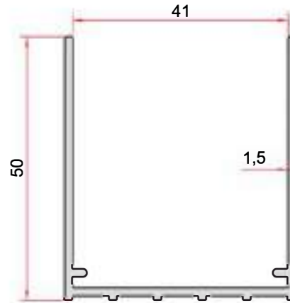
KOD-CODE EP-2636 TEORİK AĞIRLIK THEORETICAL WEIGHT 0,605 Kg/m
