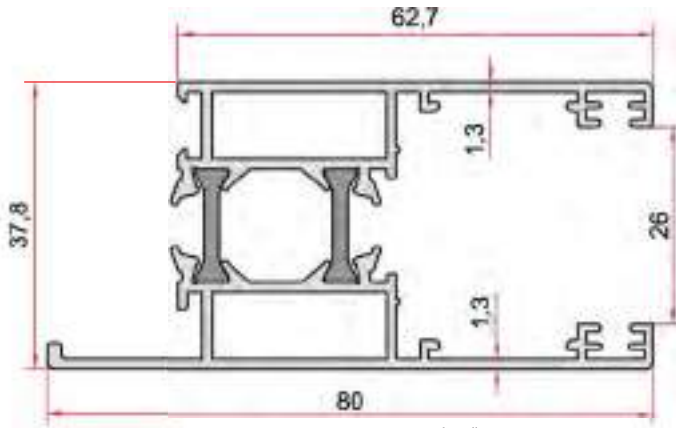
KOD-CODE TEORİK AĞIRLIK THEORETICAL WEIGHT EPSS-203-13 1,239 Kg/m
