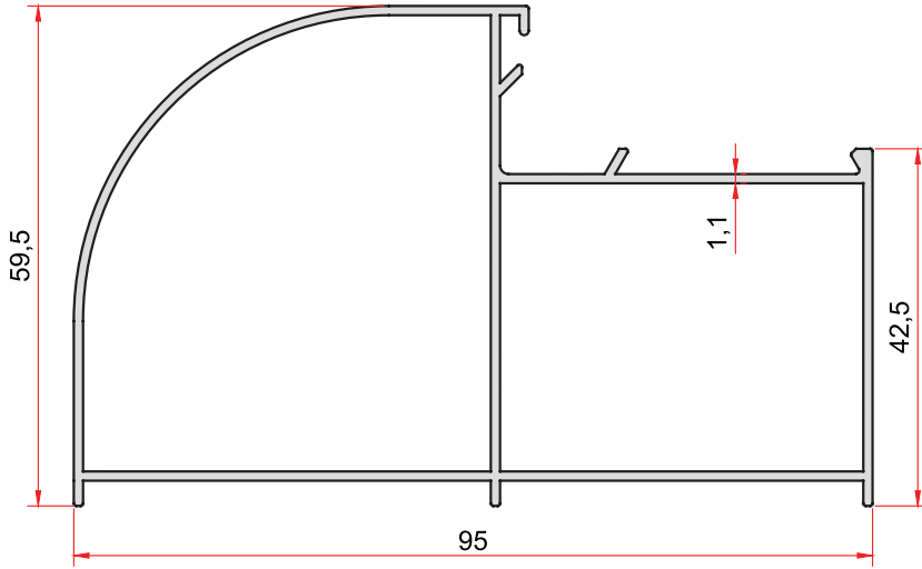
KOD-CODE TEORİK AĞIRLIK THEORETICAL WEIGHT EP-806 1,023 Kg/m
