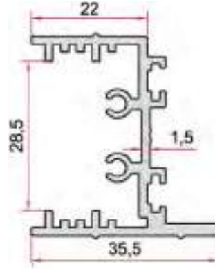
KOD-CODE TEORİK AĞIRLIK EP-2632 THEORETICAL WEIGHT 0,656 Kg/m
