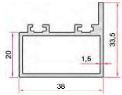
KOD-CODE TEORİK AĞIRLIK EP-2635 THEORETICAL WEIGHT 0,613 Kg/m
