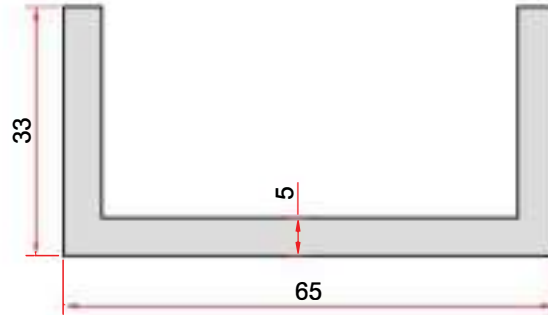
KOD-CODE TEORİK AĞIRLIK THEORETICAL WEIGHT EP-0086 1,633 Kg/m
