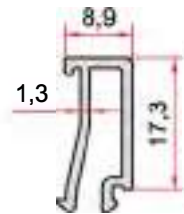
KOD-CODE TEORİK AĞIRLIK THEORETICAL WEIGHT EPSS-303-13 0,179 Kg/m
