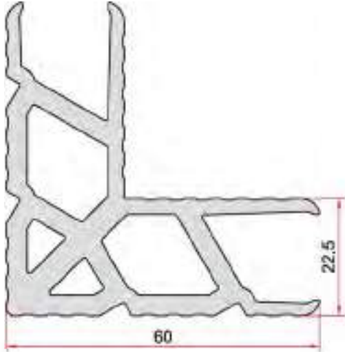
KOD-CODE TEORİK AĞIRLIK EPKT-2225-00 THEORETICAL WEIGHT 2,543 Kg/m
