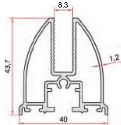
KOD-CODE TEORİK AĞIRLIK THEORETICAL WEIGHT EP-2637 0,847 Kg/m
