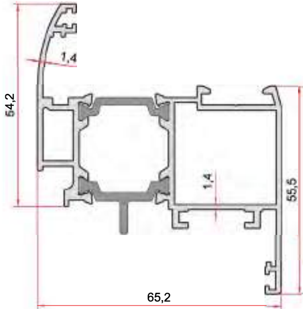
KOD-CODE TEORİK AĞIRLIK THEORETICAL WEIGHT EPİD-402-14 1,457 Kg/m
