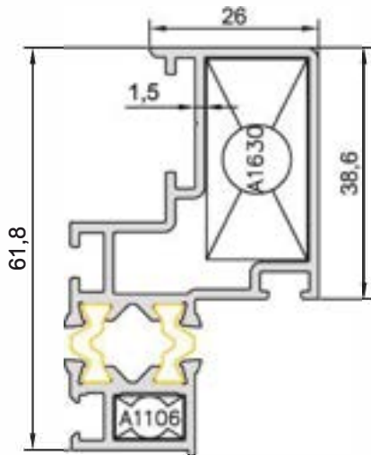
KOD-CODE AF-5072-15 TEORİK AĞIRLIK THEORETICAL WEIGHT 1,062 Kg/m
